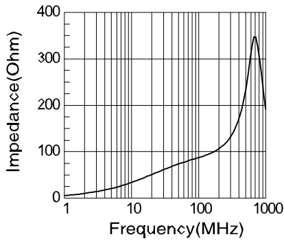
RH-3.5x5.0x0.8
